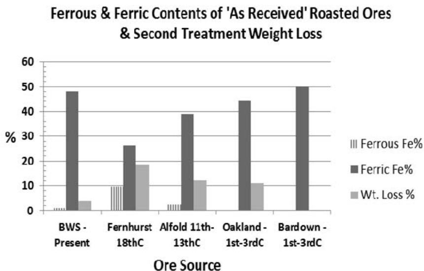
Figure 3 – ‘As Received’ Ores Ferrous/Ferric Proportions and Treatment Weight Losses
