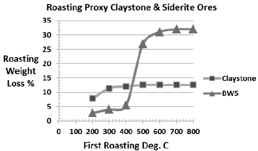
Figure 2 – Weight Loss Profiles for Wealden Claystone and Siderite Ores
