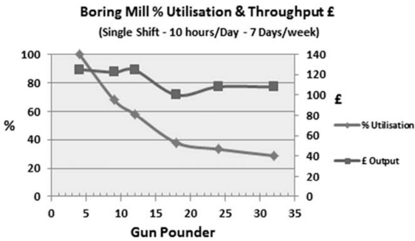
Figure 5 - Mill utilisation & weekly output value for gun size
