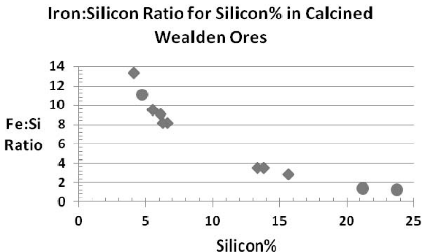
Figure 2 – Iron:Silicon Ratio for Silicon% Content in Calcined Ores
