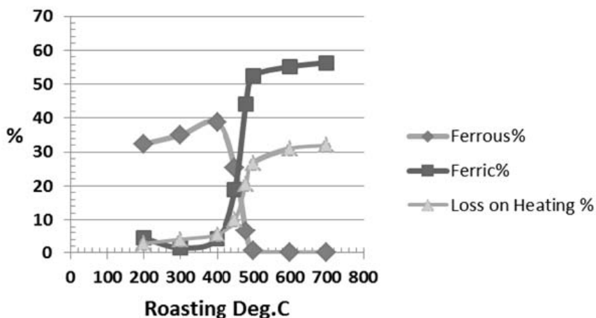
Figure 1 – Siderite Ore Ferrous to Ferric Iron Changes & Weight Loss
