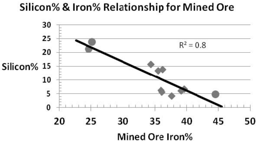
Figure 1 - Mined Ore Silicon% and Iron% Relationship
