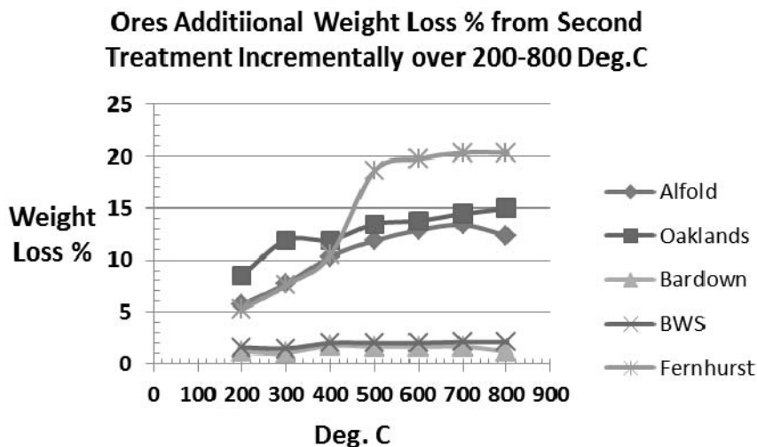
Figure 4 – Comparison of Second Treatment Weight Loss Profiles
