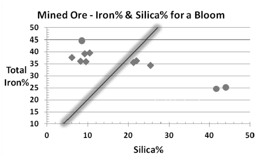
Figure 3 – Mined Ore Characteristics for Bloom production
