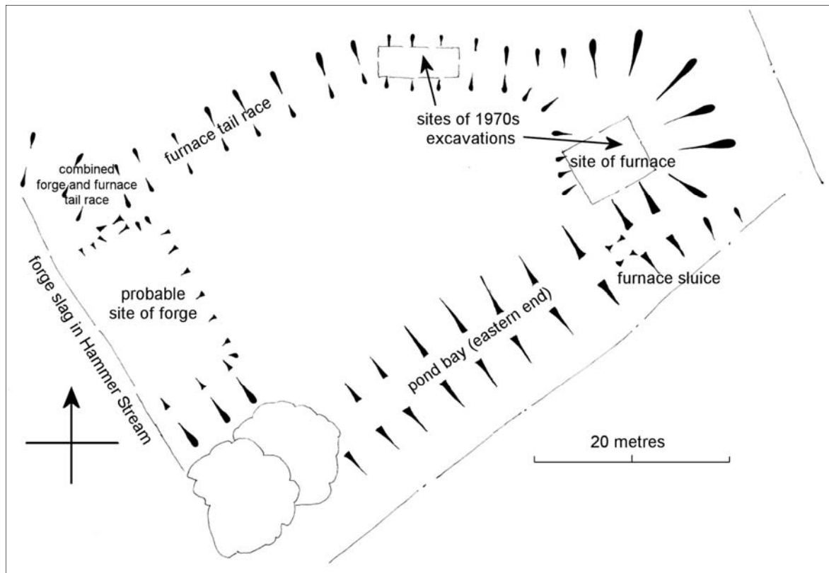
Figure 2 - Biddenden Hammer Mill furnace and forge site; 2013 plan
