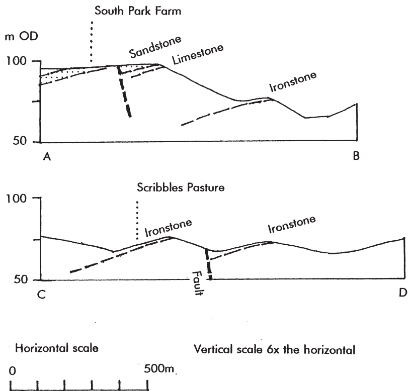
Fig 2: Geological cross-section along the lines AB and CD in Fig 1.
