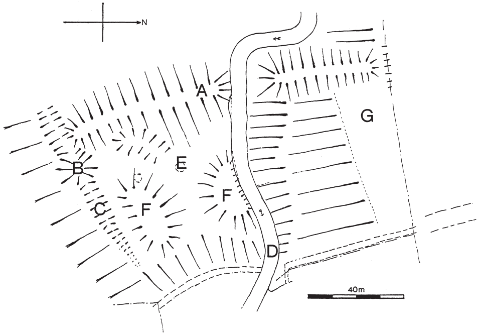
Fig 2: Plan of Iridge Furnace site
